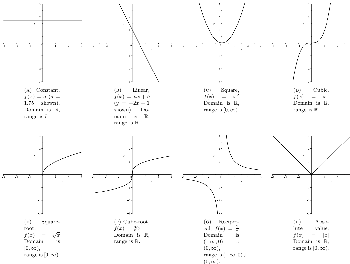
FIGURE 3. Graphs of Basic Functions You Should Know
