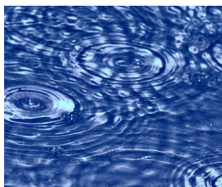
Figure 6.16 An interference pattern on the water surface is formed by interacting waves. The waves are caused by reflection of water from the rocks. (credit: modification of work by Sukanto Debnath)
