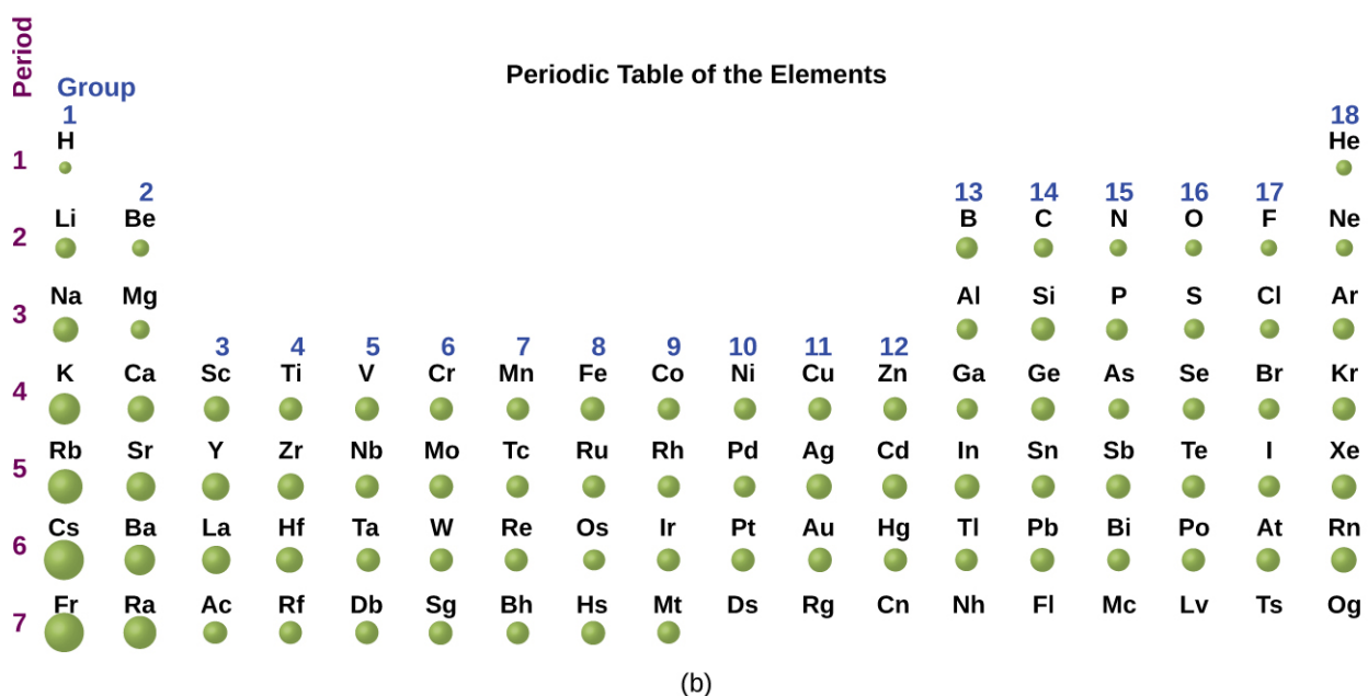
Figure 6.30 (a) The radius of an atom is defined as one-half the distance between the nuclei in a molecule consisting of two identical atoms joined by a covalent bond. The atomic radius for the halogens increases down the group as n increases. (b) Covalent radii of the elements are shown to scale. The general trend is that radii increase down a group and decrease across a period.
