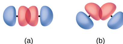
Figure 8.3 (a) The overlap of two p orbitals is greatest when the orbitals are directed end to end. (b) Any other arrangement results in less overlap. The dots indicate the locations of the nuclei.
