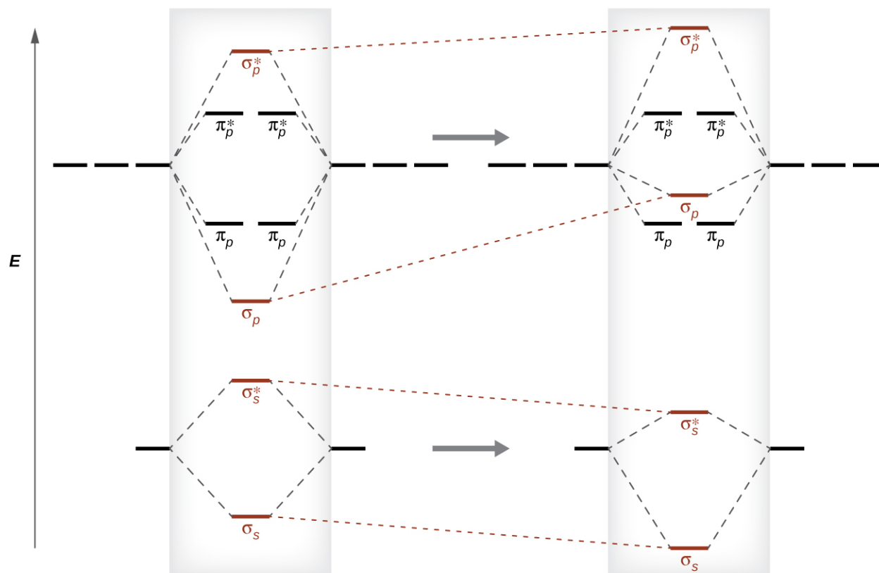
Figure 8.38 Without mixing, the MO pattern occurs as expected, with the \sigma_p orbital lower in energy than the \pi_p orbitals. When s-p mixing occurs, the orbitals shift as shown, with the \sigma_p orbital higher in energy than the \pi_p orbitals.
