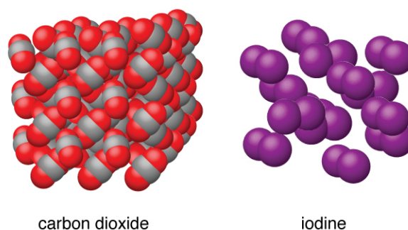
Figure 10.42 Carbon dioxide (CO 2 ) consists of small, nonpolar molecules and forms a molecular solid with a melting point of -78^{\circ}\text{C} . Iodine (I 2 ) consists of larger, nonpolar molecules and forms a molecular solid that melts at 114^{\circ}\text{C} .
