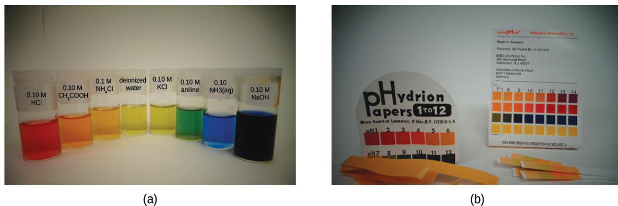
Figure 14.5 (a) A solution containing a dye mixture, called universal indicator, takes on different colors depending upon its pH. (b) Convenient test strips, called pH paper, contain embedded indicator dyes that yield pH-dependent color changes on contact with aqueous solutions. (credit: modification of work by Sahar Atwa)
